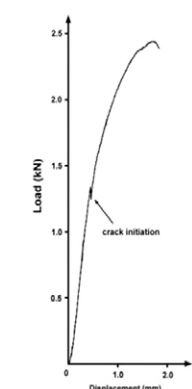
Fig. 2. Load vs displacement curve of EXZRTS group.
