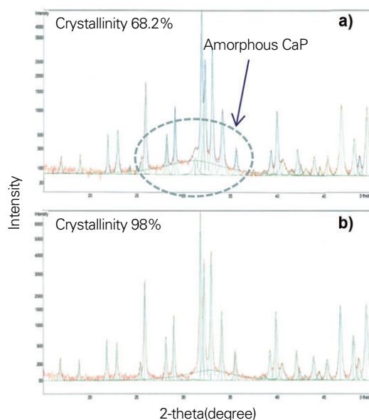
Fig. 2. The comparison of the X-ray diffraction pattern of HA special processing. Before (a) and after (b).
