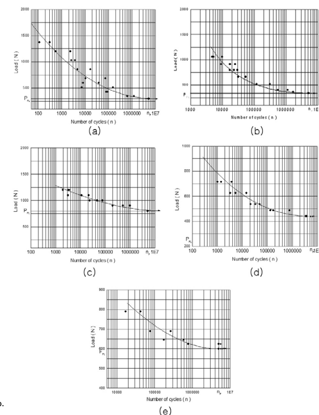
Fig. 3. Fatigue load vs cycles to failure of each experimental group: (a)EXTNTS, (b)EXANTS, (c) EXZRTS, (d) INTIWS, (e) INTICS.
